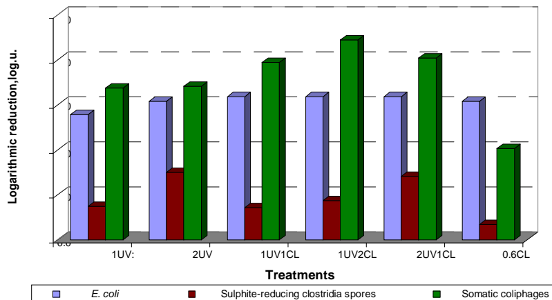
Figure 5. Logarithmic reductions in E. coli , sulphite-reducing clostridia spores and somatic coliphages for the disinfection treatments evaluated in the study.
